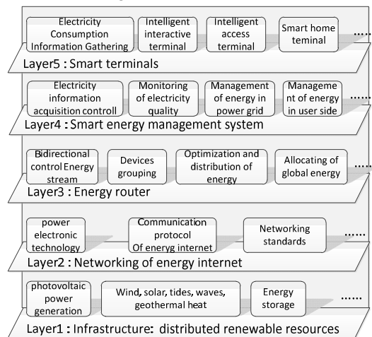
Fig. 4 System architecture of energy internet
